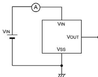
Circuit 2
