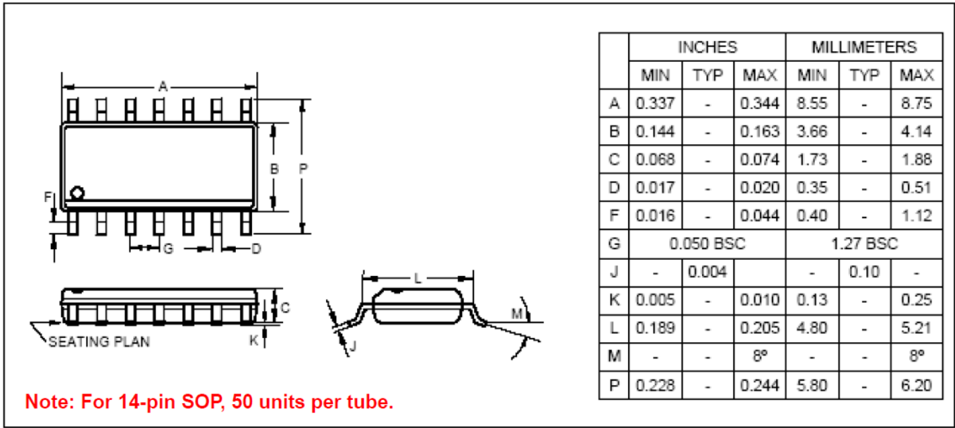
14-Pin Plastic SOP (150 mil)
